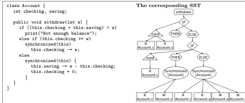
Fig. 3. An example of a static summary tree (SST), where Account.c and Account.s denote Account.checking and Account.saving , and “R” or “W” denotes that the node is a read or write, respectively.
